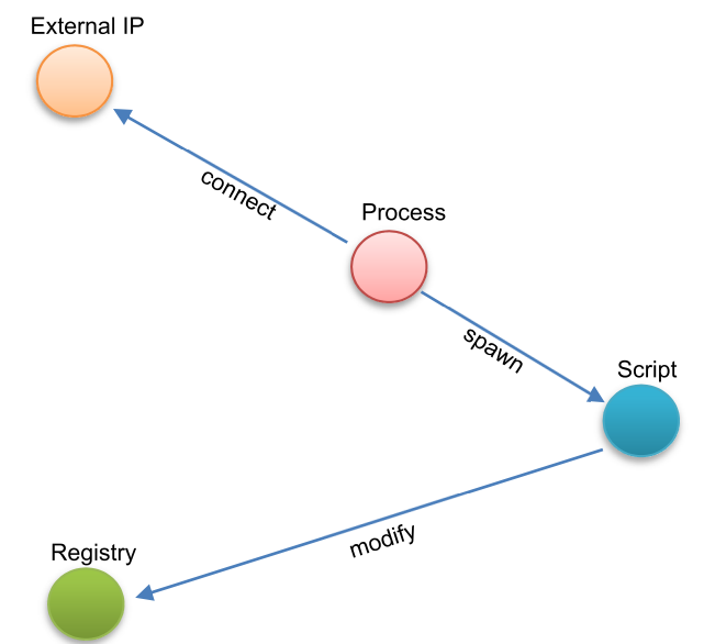
FIGURE 2. Visualization of a malicious subgraph captured by the proposed framework. Nodes represent processes, files, registry keys, and network entities; edges denote behavioral interactions indicating multi-hop APT activities.
