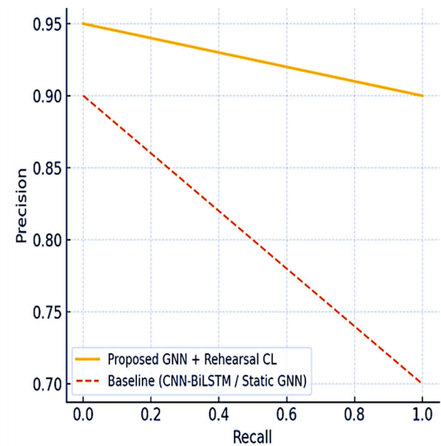
FIGURE 1. Precision–Recall curve showing that the proposed GNN with rehearsal-based continual learning maintains high precision and recall under class imbalance, outperforming baseline models.
